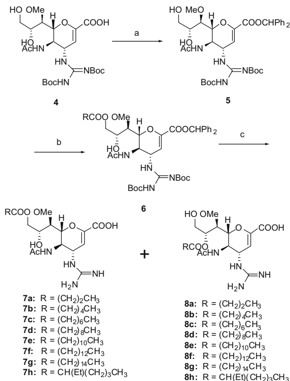
Scheme 1. Reagents: (a) Ph 2 CN 2 , THF (85%); (b) RCOCl (1.1 equiv), TEA (1.2 equiv), CH 2 Cl 2 , (50–70%); (c) CF 3 COOH–CH 2 Cl 2 (60–70%).
