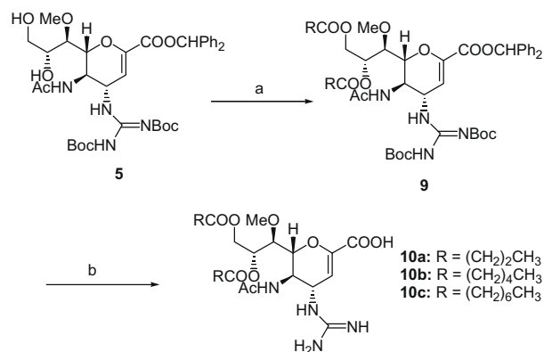
Scheme 2. Reagents: (a) RCOCl (3.0 equiv), TEA (3.0 equiv), 4- N,N -dimethylaminopyridine (3.0 equiv), CH 2 Cl 2 (80–90%); (b) CF 3 COOH–CH 2 Cl 2 (60–70%).
