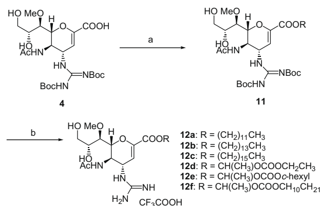
Scheme 3. Reagents and conditions: (a) (i) KOH (1.1 equiv), MeOH, (ii) 12a–12c : RBr (1.1 equiv), DMF 50 °C, 4 h (50–80%); 12d–12f : ICH(CH 3 )OCOOR (1.5 equiv), DMF, 20 °C, 1 h (50–60%); (b) CF 3 COOH–CH 2 Cl 2 (60–70%).
